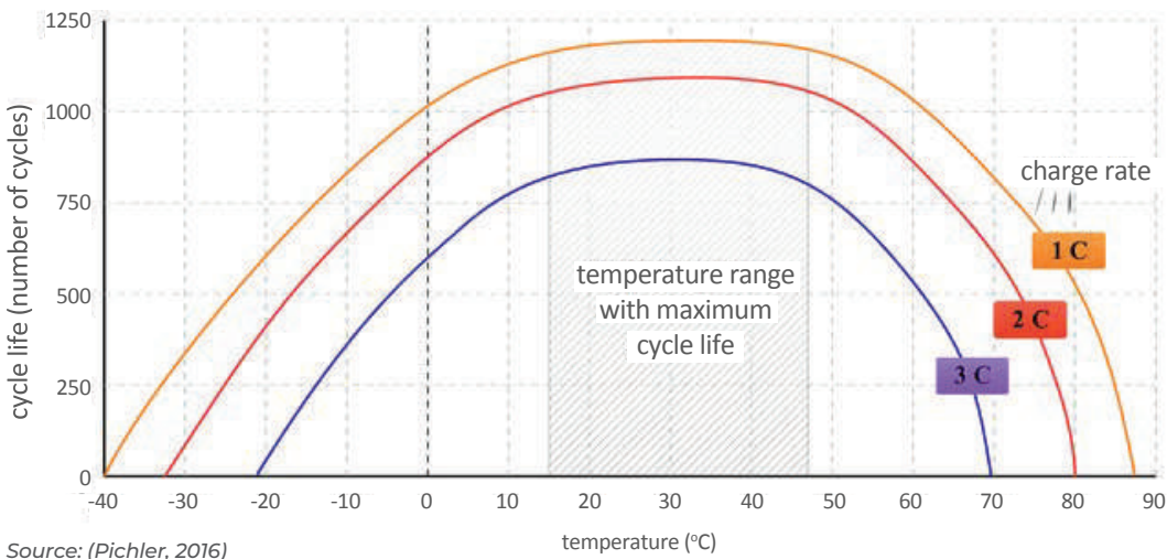
Figure 13 Effect of charge rate and temperature on the cycle life of the battery.
