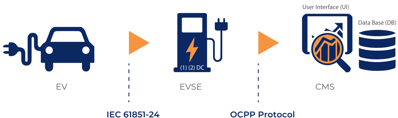
Figure 15 Communication protocol between EV and Central Management System (CMS) for fast chargers
